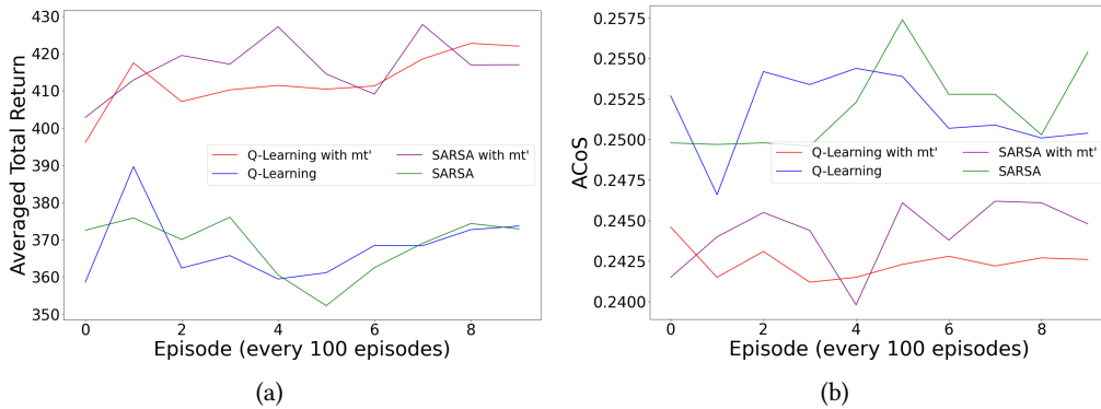
Figure 4: Comparisons between the performances of Q-learning and Sarsa, both with and without the changing epsilon ( mt' ) in a dynamic environment. (a): The average total return per 100 episodes. (b): The ACoS calculated based on the given formulation in Section 2.2.
